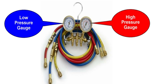
Figure 3. Gauge Manifold Set.
